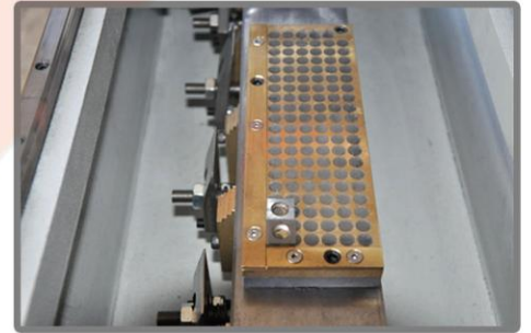
Optional Magnetic Attachment For Replacable Inserts
